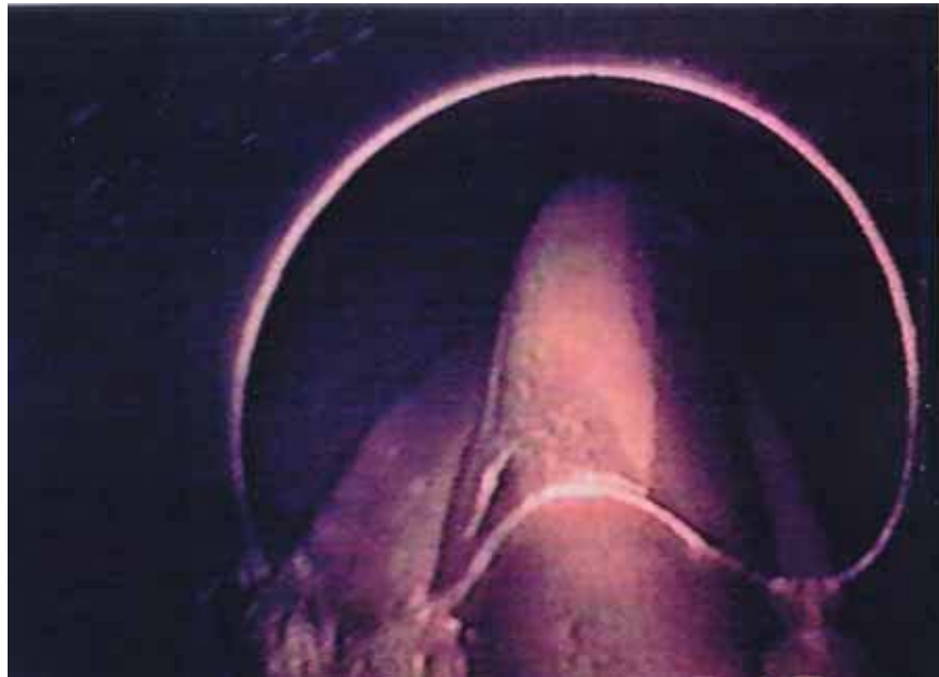
Figure B-19. —View of interior of deformed HDPE pipe from CCTV camera.
