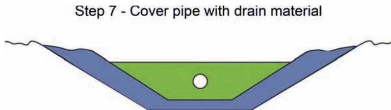
Figure 74. —Place remaining drain material.
