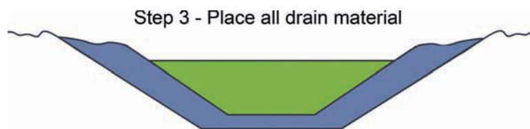
Figure 70.—Drain material placement.
